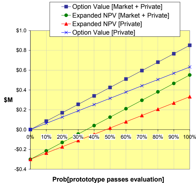
FIGURE 14. Sensitivity analysis for the MathWizards project.
