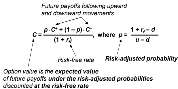
FIGURE 12. Risk-neutral valuation in the binomial model.
