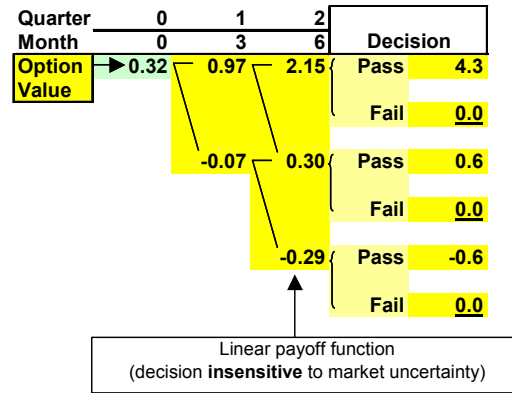
FIGURE 13. Reduced decision tree for the MathWizards project. The full development decision is insensitive to market uncertainty.
