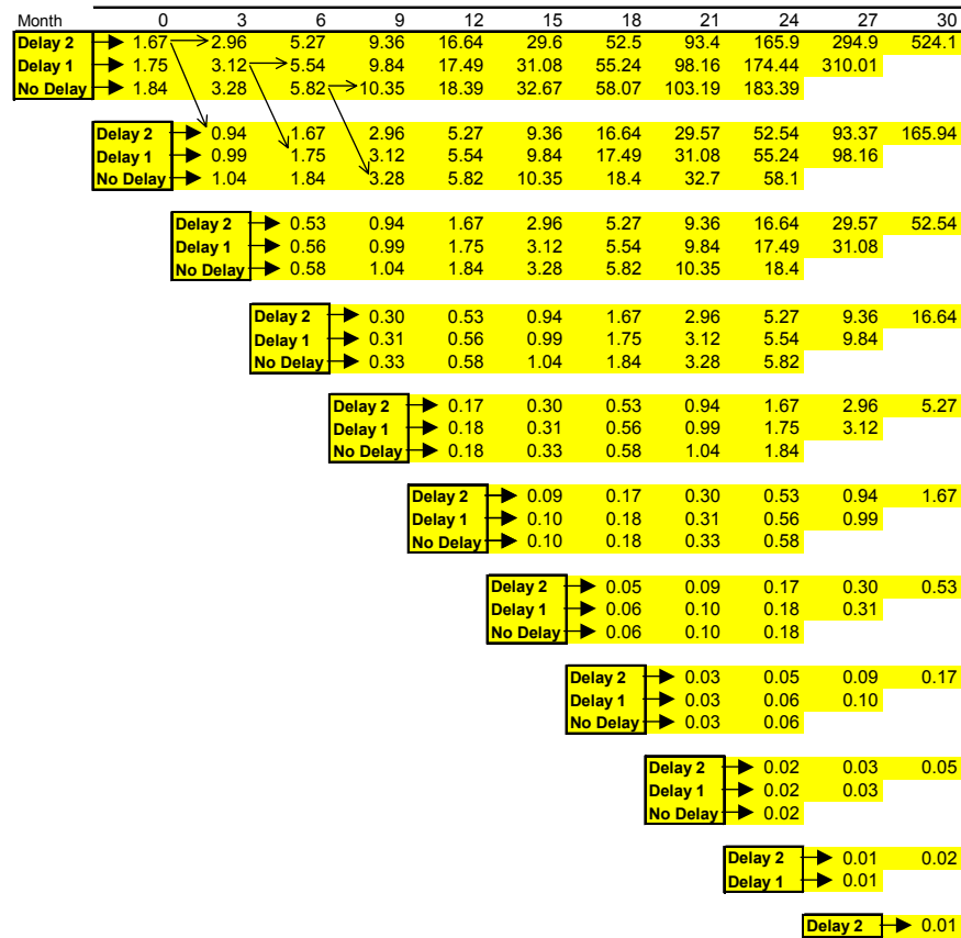
FIGURE 10. A binomial lattice for MathWizards' market payoff.
