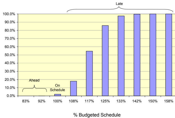
FIGURE 7. Completion probability estimates for Stage 2.
